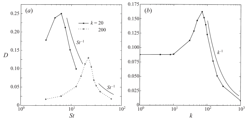
FIGURE 15. Long-time drop response in an RE flow at Re = 1.0 with varying (a) frequency; (b) interfacial tension, St = 4\pi .
