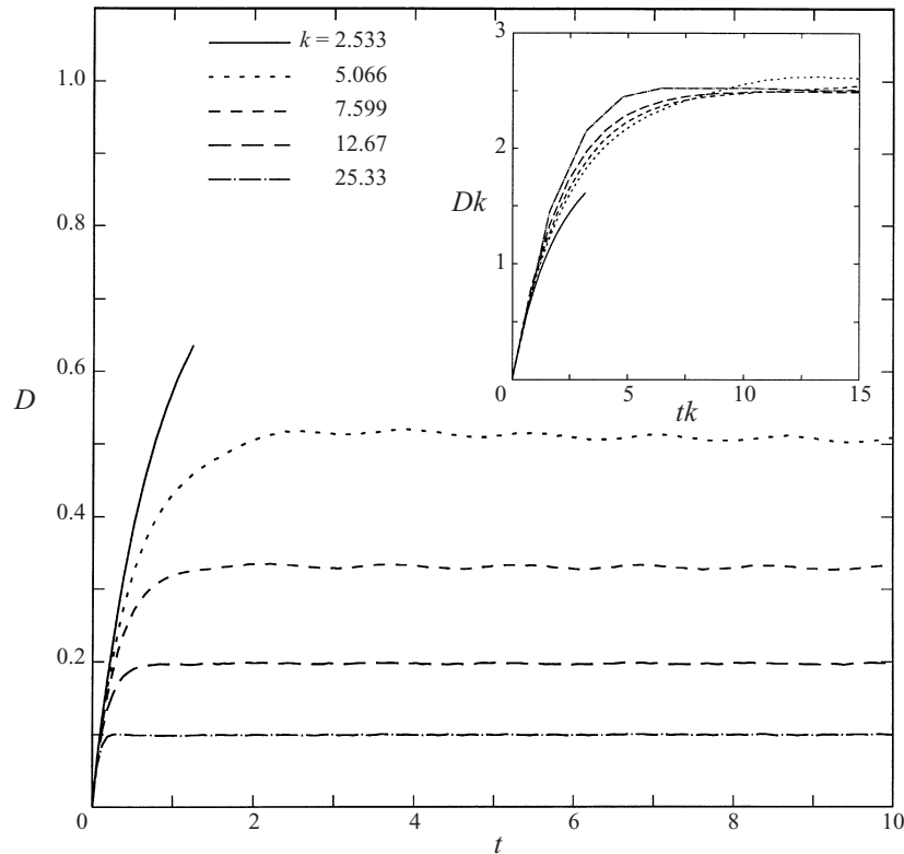
FIGURE 4. Effect of interfacial tension on drop deformation in a potential vortex at Re = 0.1 . Inset shows the same in scaled variables.
