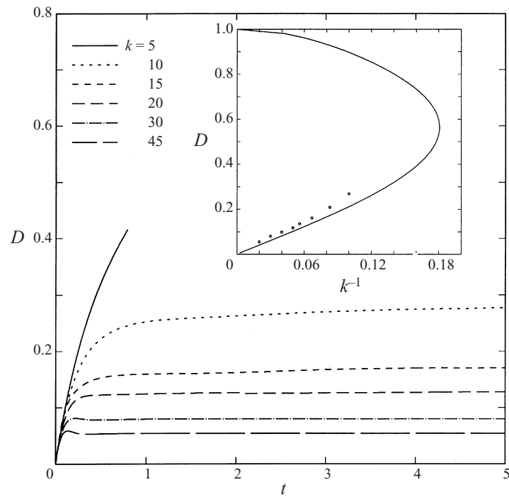
FIGURE 8. Effect of interfacial tension on drop deformation in a steady extensional (RE with St = 0 ) flow at Re = 0.1 . In the inset we show comparison with the analytical Stokes flow results from Buckmaster & Flaherty (1973) for the long-time drop response.
