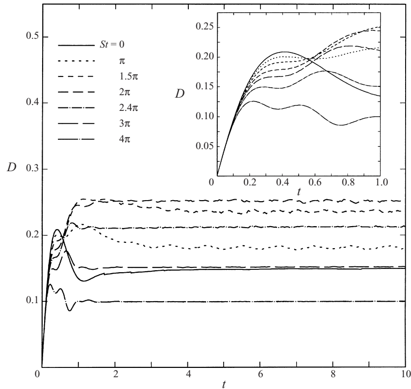
FIGURE 14. Effect of frequency on drop deformation in an RE flow at Re = 1.0 and k = 20 . Inset shows a magnification at small times.
