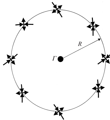
FIGURE 1. Velocity gradient in a potential vortex.
