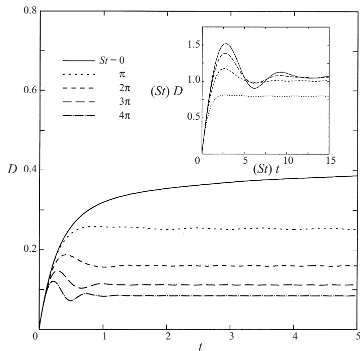
FIGURE 9. Effect of frequency on drop deformation in an RE flow at Re = 0.1 and k = 8.0 . Inset shows the same in scaled variables.
