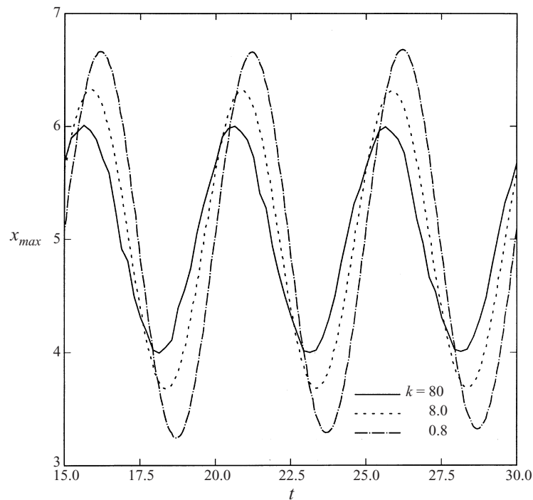
FIGURE 10. Effect of interfacial tension on the phase lag of the drop response in an RE flow at Re = 0.1 and St = 0.8\pi .
