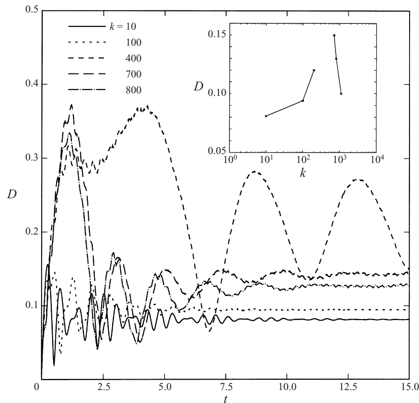
FIGURE 18. Effect of interfacial tension on drop deformation in an RE flow at Re = 10 and St = 4\pi . In the inset long-time drop response for varying tension is shown.
