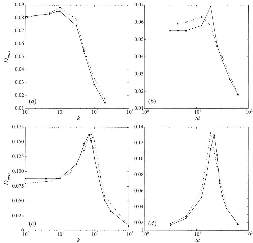
FIGURE 20. Long-time drop responses for RE (solid) and OE (dotted) flows for varying (a) interfacial tension at Re = 0.1 , St = 4\pi ; (b) frequency at Re = 0.1 , k = 45 ; (c) interfacial tension at Re = 1.0 , St = 4\pi ; (d) frequency at Re = 1.0 , k = 200 .
