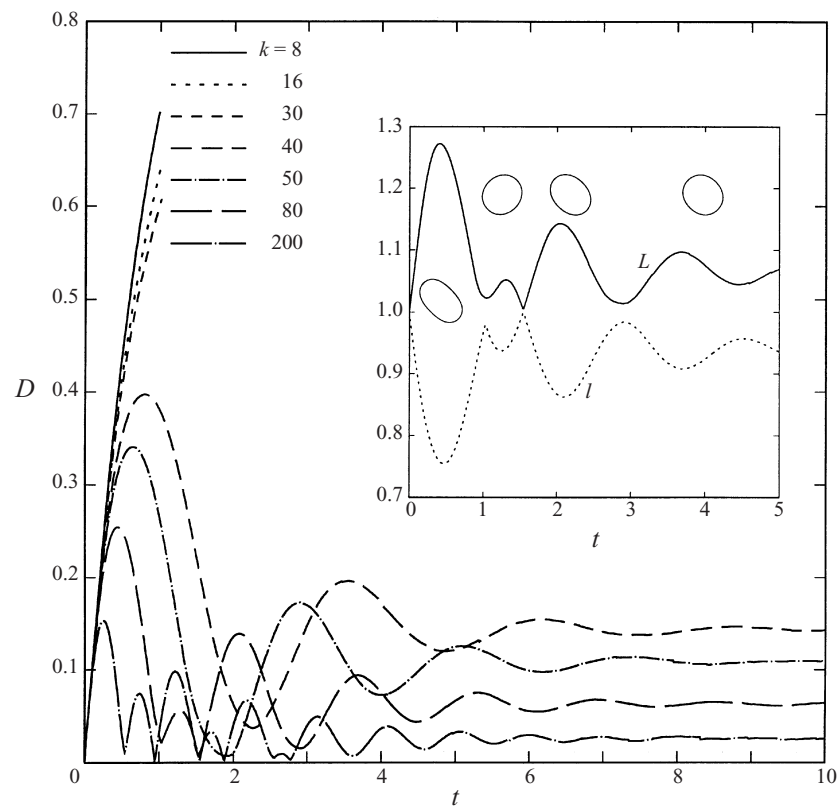
FIGURE 16. Effect of interfacial tension on drop deformation in a steady extensional (RE with St = 0 ) flow at Re = 10.0 . Inset shows evolution of maximum (solid) and minimum (dotted) distances of the drop interface from its centre for k = 80 . Also the drop shapes at t = 0.5, 1.32, 2.04 and 4.09 are shown. Their positions approximately correspond to the time axis.
