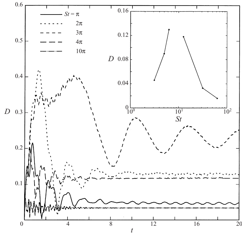
FIGURE 17. Effect of frequency on drop deformation in an RE flow at Re = 10 and k = 200 . Inset shows long-time drop response for varying frequency.
