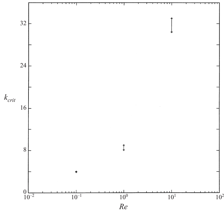
FIGURE 7. Effect of Reynolds number on the critical value of k in a potential vortex. The upper and the lower bounds indicate the closest values of k for which a bounded and an unbounded shape, respectively, are numerically found at that Re .
