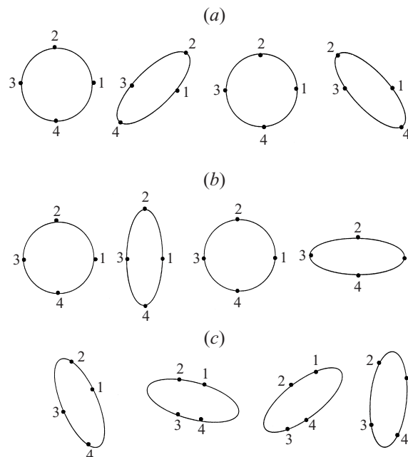
FIGURE 2. Drops in different time-periodic linear flows: (a) oscillatory shear flow, (b) oscillatory extensional (OE) flow, and (c) vortex/generalized rotating extensional (RE) flow.
