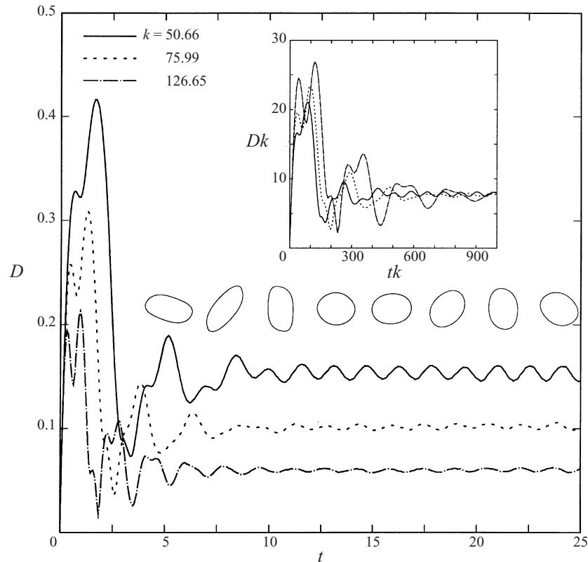
FIGURE 6. Effect of interfacial tension on drop deformation in a potential vortex at Re = 10.0 . Inset shows the same in scaled variables. Drop shapes for k = 50.66 at t = 0.69, 1.51, 2.27, 3.13, 3.85, 4.67, 5.42 and 6.24 (from left to right), during the initial transient. The shape positions in the figure do not correspond to the time axis.
