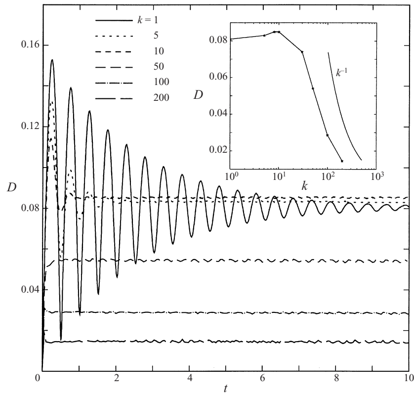
FIGURE 11. Effect of interfacial tension on drop deformation in an RE flow at Re = 0.1 and St = 4\pi . Inset shows long-time drop response for varying tension.
