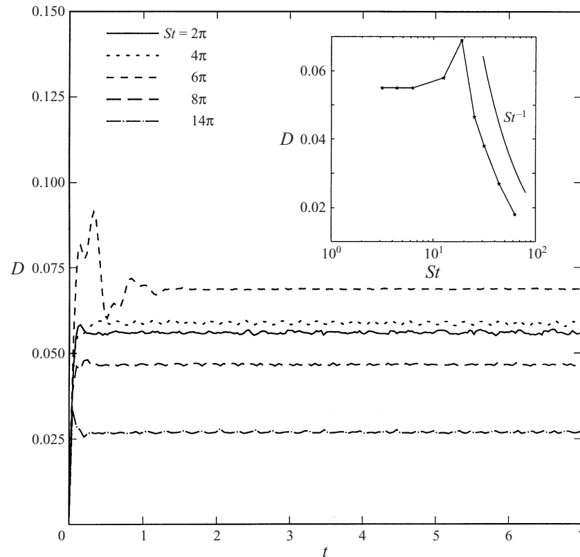
FIGURE 12. Effect of frequency on drop deformation in an RE flow at Re = 0.1 and k = 45.0 . Inset shows long-time drop response for varying frequency.
