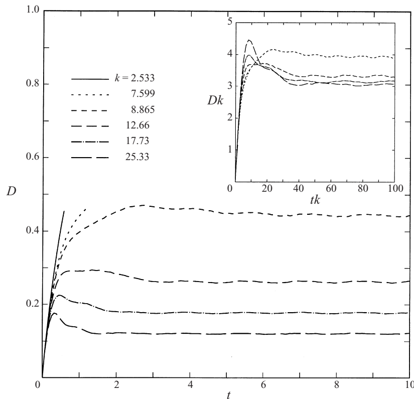
FIGURE 5. Effect of interfacial tension on drop deformation in a potential vortex at Re = 1.0 . Inset shows the same in scaled variables.
