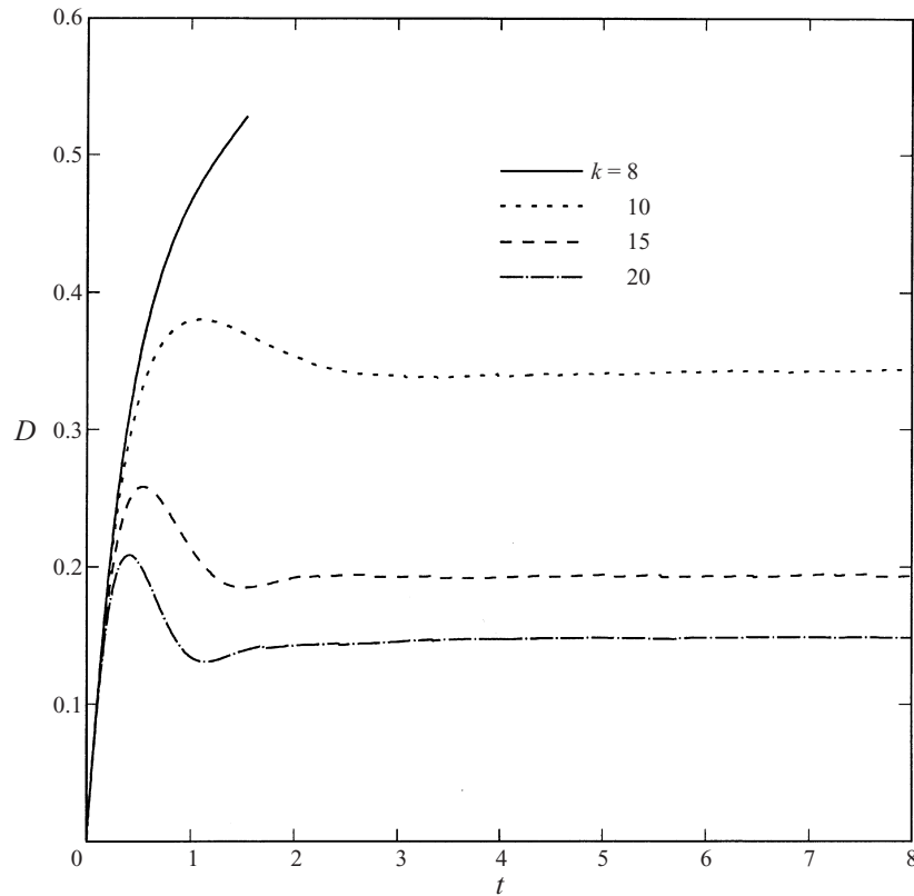
FIGURE 13. Effect of interfacial tension on drop deformation in a steady extensional (RE with St = 0 ) flow at Re = 1.0 .
