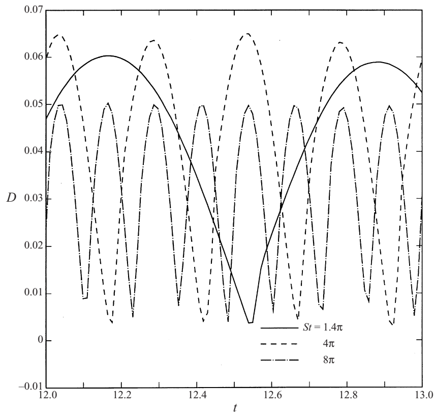
FIGURE 19. Effect of frequency on drop deformation in an OE flow at Re = 0.1 and k = 45 .
