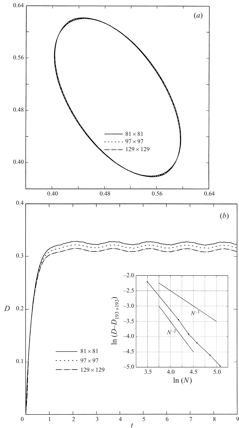
FIGURE 3. For caption see facing page.
